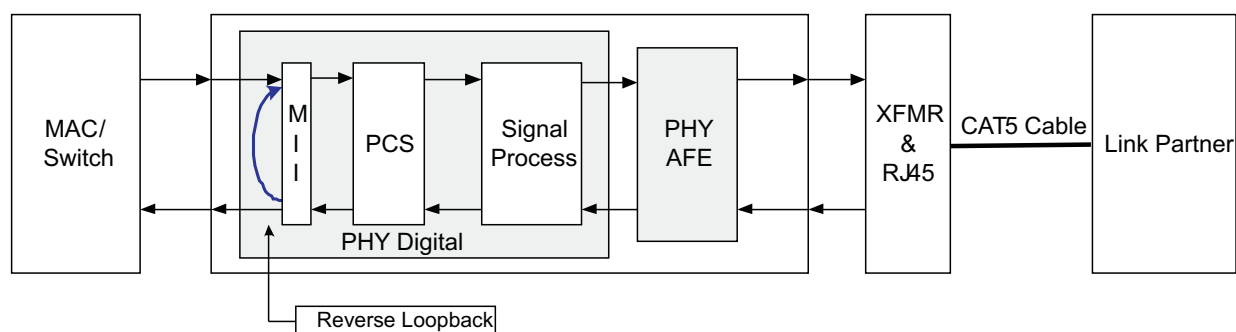
Figure 3-6. Block Diagram, Far-End Loopback Mode
