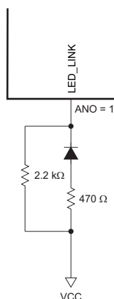
Figure 3-4. AN Pin Configuration and LED Loading Example
