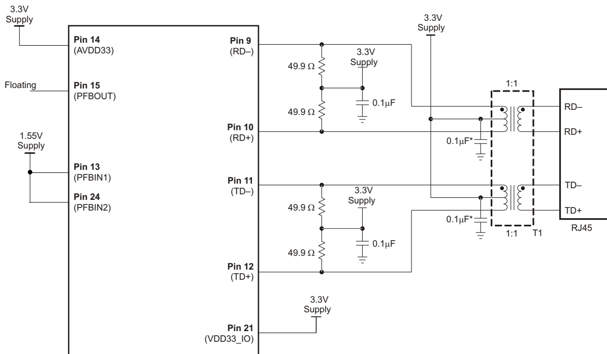
Figure 3-2. Power Connections for Dual Supply Operation
