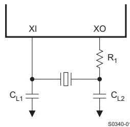
Figure 7-2. Crystal Oscillator Circuit
