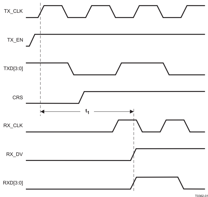
Figure 9-22. 10Mbps Internal Loopback Timing
