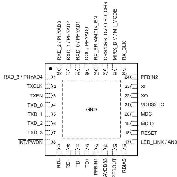
Figure 2-1. TLK10x PIN DIAGRAM, TOP VIEW
