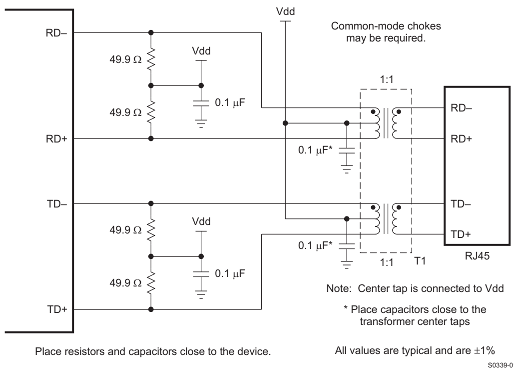
Figure 7-1. 10/100Mbps Twisted Pair Interface
