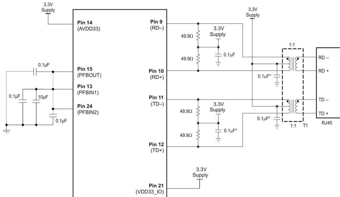
Figure 3-1. Power Connections for Single Supply Operation
