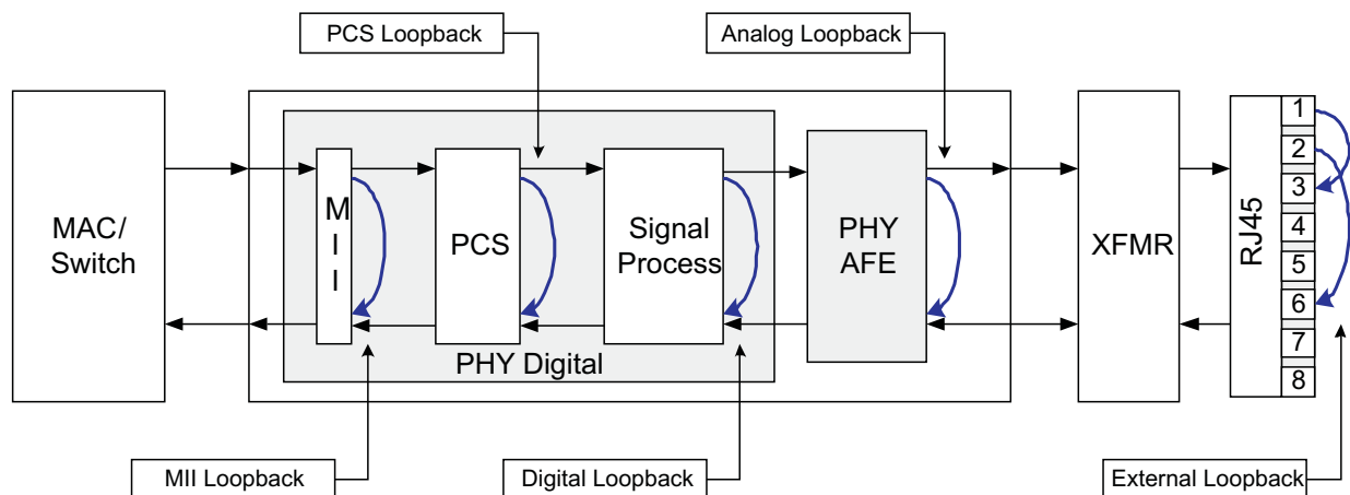
Figure 3-5. Block Diagram, Near-End Loopback Mode
