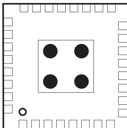
Figure 7-3. Example Layout
