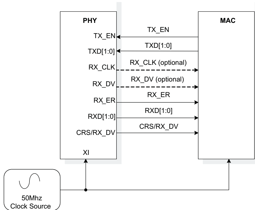
Figure 4-2. TLK10x RMII/MAC Connection
