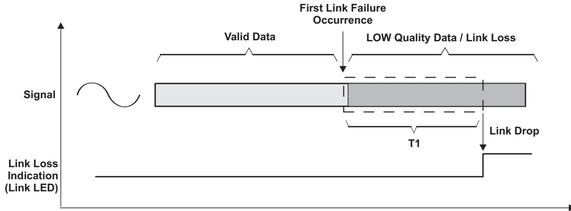
Figure 5-3. TLK10x Link Loss Mechanism
